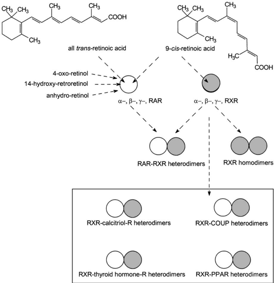
Figure 2.6. Interactions of all- trans - and 9- cis -retinoic acids (and other active retinoids) with retinoid receptors. COUP, chicken ovalbumin upstream promoter.
