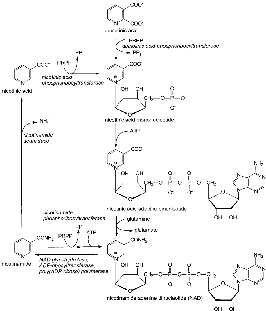
Figure 8.2. Synthesis of NAD from nicotinamide, nicotinic acid, and quinolinic acid. Quinolinic acid phosphoribosyltransferase, EC 2.4.2.19; nicotinic acid phosphoribosyltransferase, EC 2.4.2.11; nicotinamide phosphoribosyltransferase, EC 2.4.2.12; nicotinamide deamidase, EC 3.5.1.19; NAD glycohydrolase, EC 3.2.2.5; NAD pyrophosphatase, EC 3.6.1.22; ADP-ribosyltransferases, EC 2.4.2.31 and EC 2.4.2.36; and poly(ADP-ribose) polymerase, EC 2.4.2.30. PRPP, phosphoribosyl pyrophosphate.
