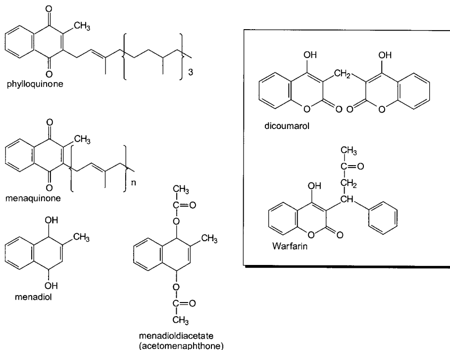
Figure 5.1. Vitamin K vitamers and the vitamin K antagonists dicoumarol and warfarin. Relative molecular masses ( M_r ): phyloquinone, 450.7; menaquinone-4, 447.4; menaquinone-5, 512.8; menaquinone-6, 580.0; menaquinone-7, 649.0; menaquinone-8, 717.1; menadione, 172.2; menadiol diacetate, 258.3; dicoumarol, 336.3; and warfarin 308.3.
