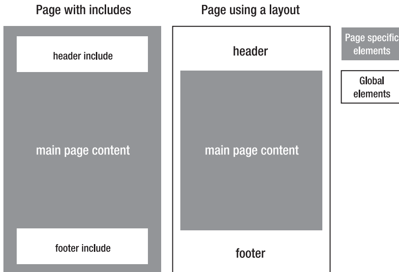
Figure 9-2. The differences between includes and layouts
