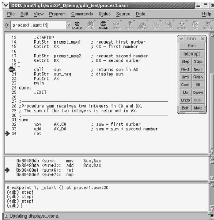
Figure C.5 DDD window after single stepping from the breakpoint on line 20.
