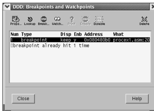
Figure C.3 Breakpoints window.
