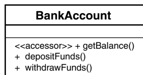
FIGURE 8.5 A stereotype that qualifies the operation.
