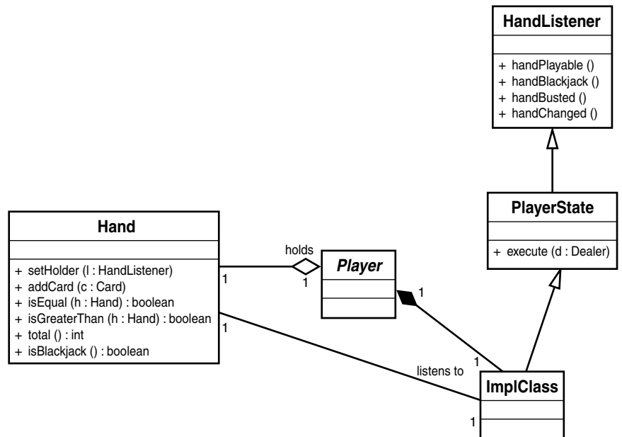
FIGURE 16.6 The State framework class diagram.
