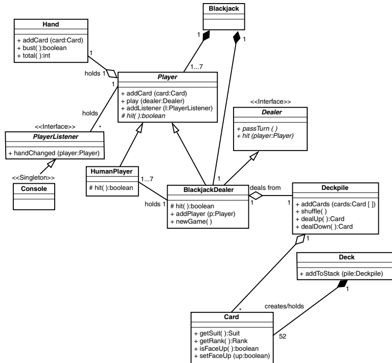
FIGURE 15.12 The Blackjack class model.
