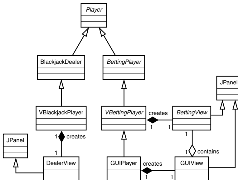
FIGURE 19.3 The Player abstraction hierarchy.
