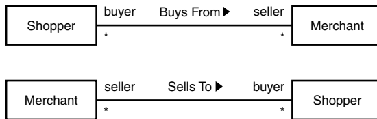
FIGURE A.4 The Shopper/Merchant Association.
