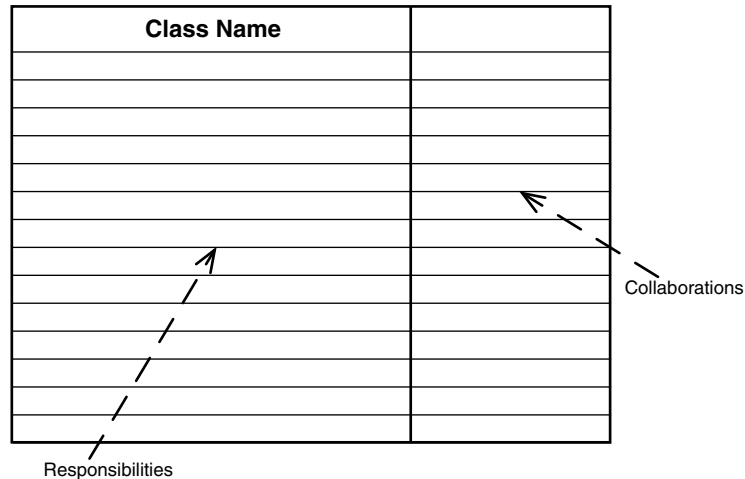
FIGURE 10.2 A CRC card template.
