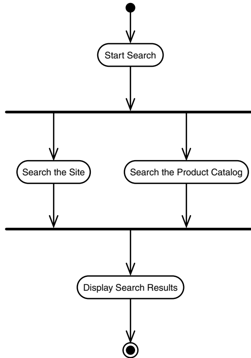
FIGURE 9.11 The Search Activity diagram.
