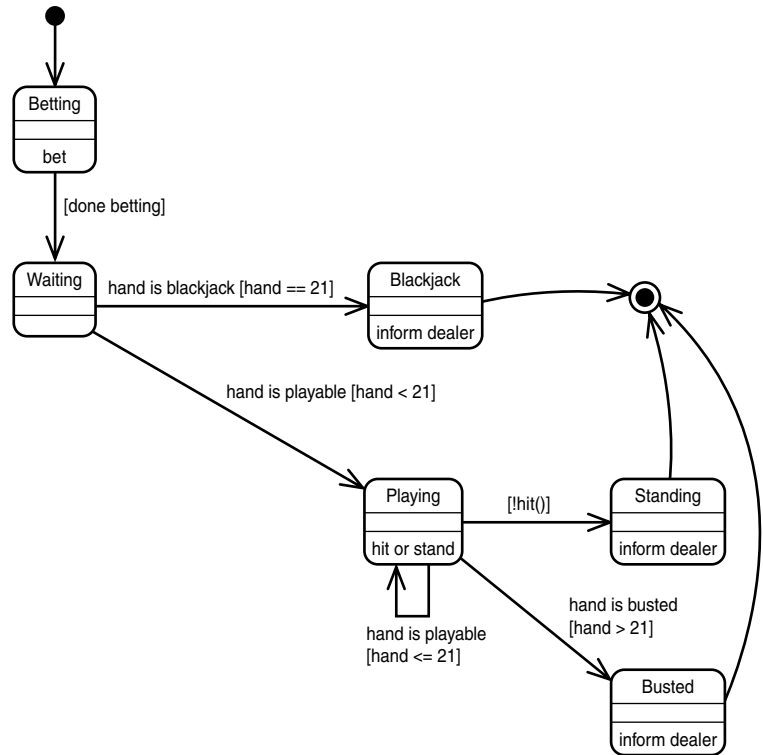
FIGURE 17.5 The state diagram for the players.
