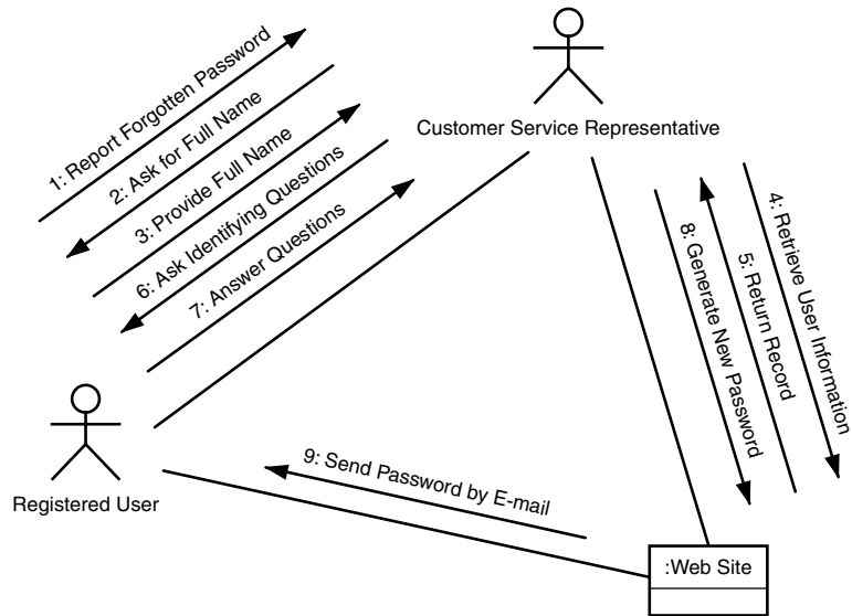
FIGURE 9.10 The Forgot Password collaboration diagram.
