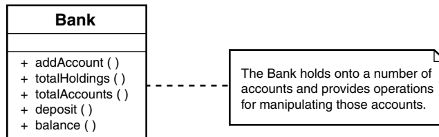
FIGURE 8.4 A detailed example of a note.
