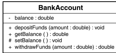
FIGURE 8.3 A fully described class.
