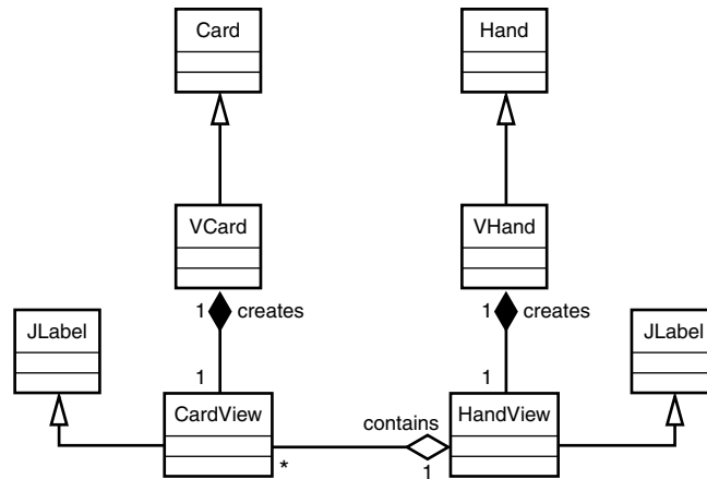
FIGURE 19.4 The Hand and Card abstraction hierarchy.
