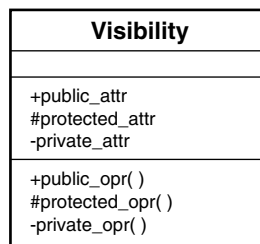
FIGURE C.2 Method and attribute visibility.
