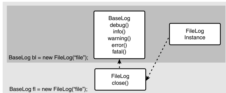
FIGURE 6.2 Different views of the same object.
