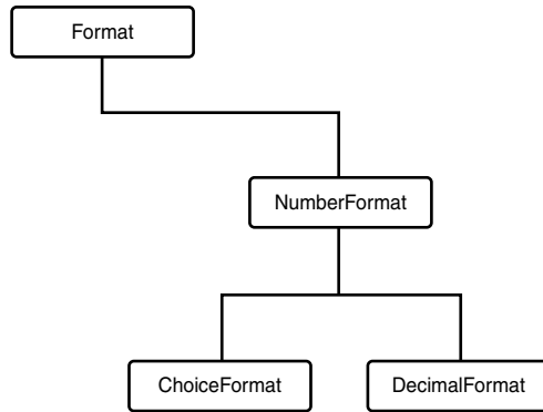
FIGURE 4.8 DecimalFormat is a descendant of Format.
