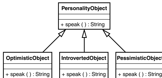
FIGURE A.6 The PersonalityObject Hierarchy.
