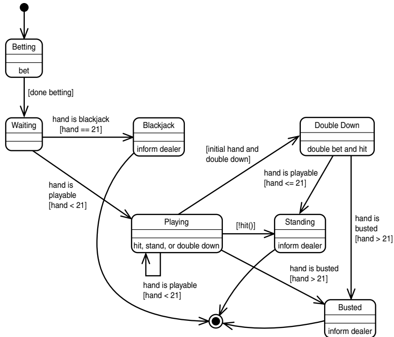
FIGURE A.7 The updated BettingPlayer state diagram.
