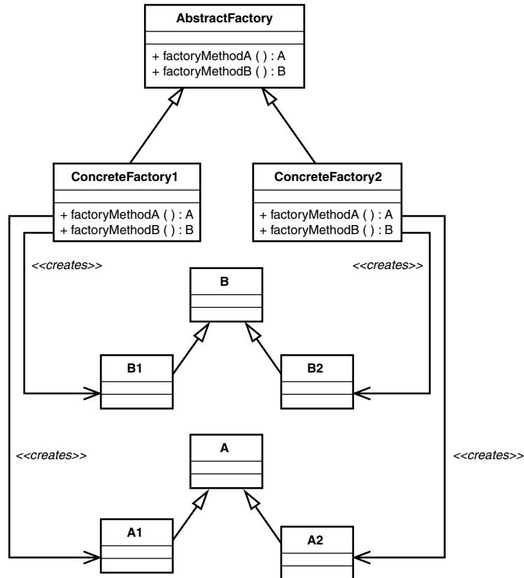
FIGURE 12.1 The Abstract Factory Pattern.
