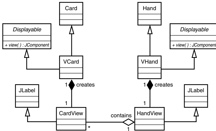
FIGURE 19.6 The updated Hand and Card abstraction hierarchy.
