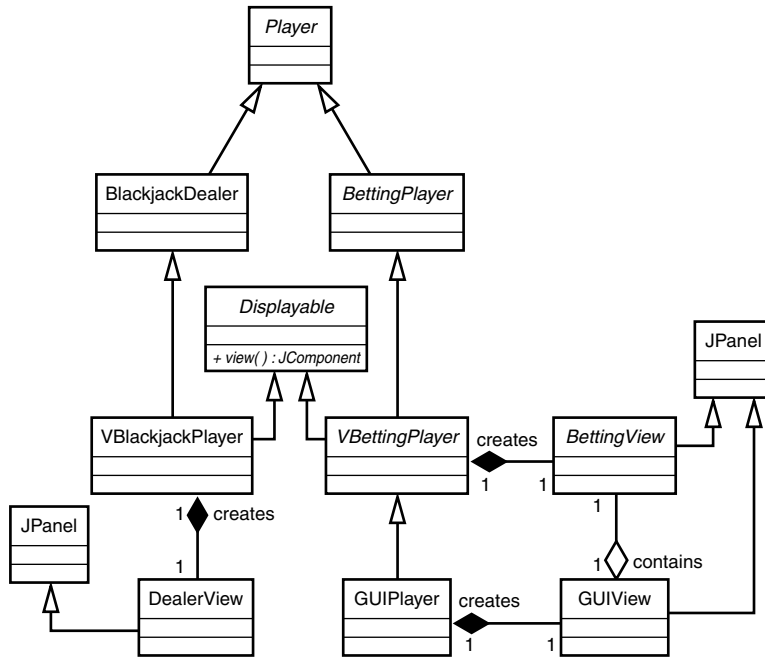
FIGURE 19.5 The updated Player abstraction hierarchy.
