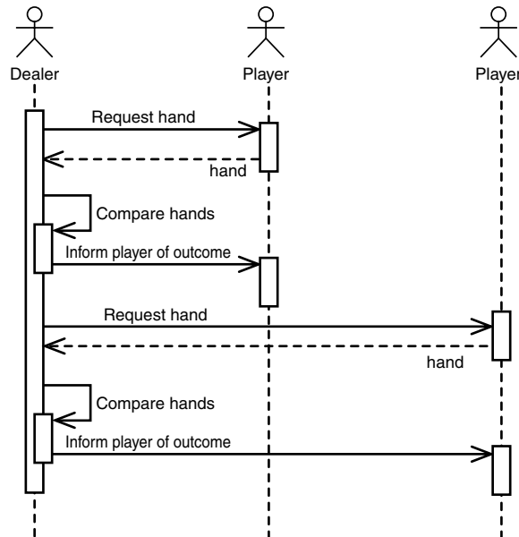
FIGURE 16.1 The sequence diagram for Dealer Fulfills Game use case.
