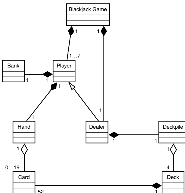
FIGURE 17.1 The Blackjack domain model.
