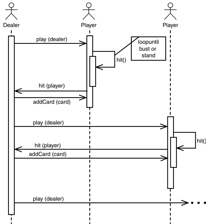
FIGURE 15.14 The procedural interaction between players and the dealer.
