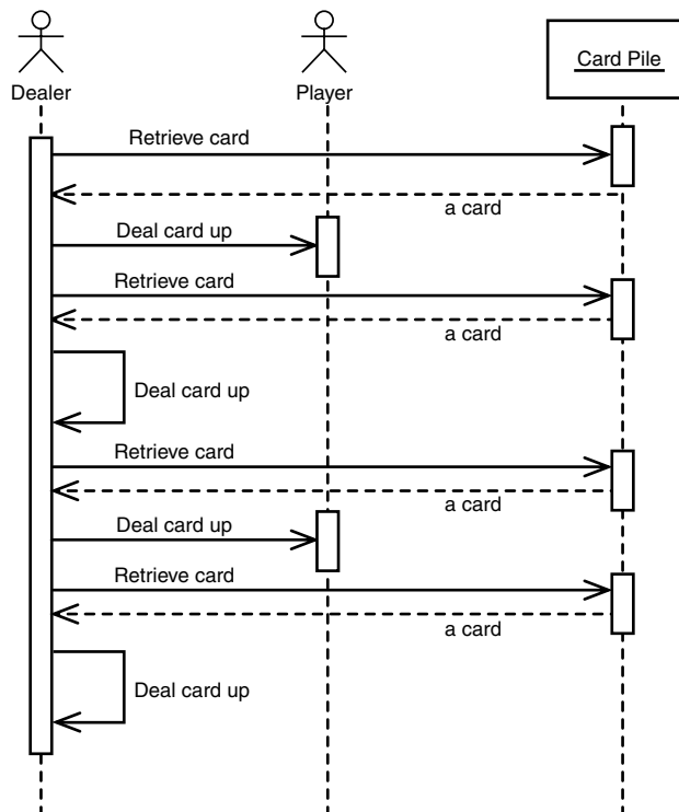
FIGURE 15.2 The sequence diagram for Deal Cards use case.
