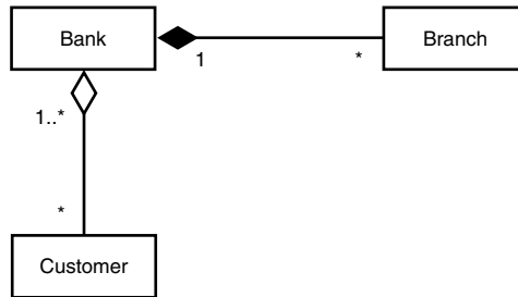
FIGURE 8.14 The Bank in an aggregation and composition relationship at the same time.
