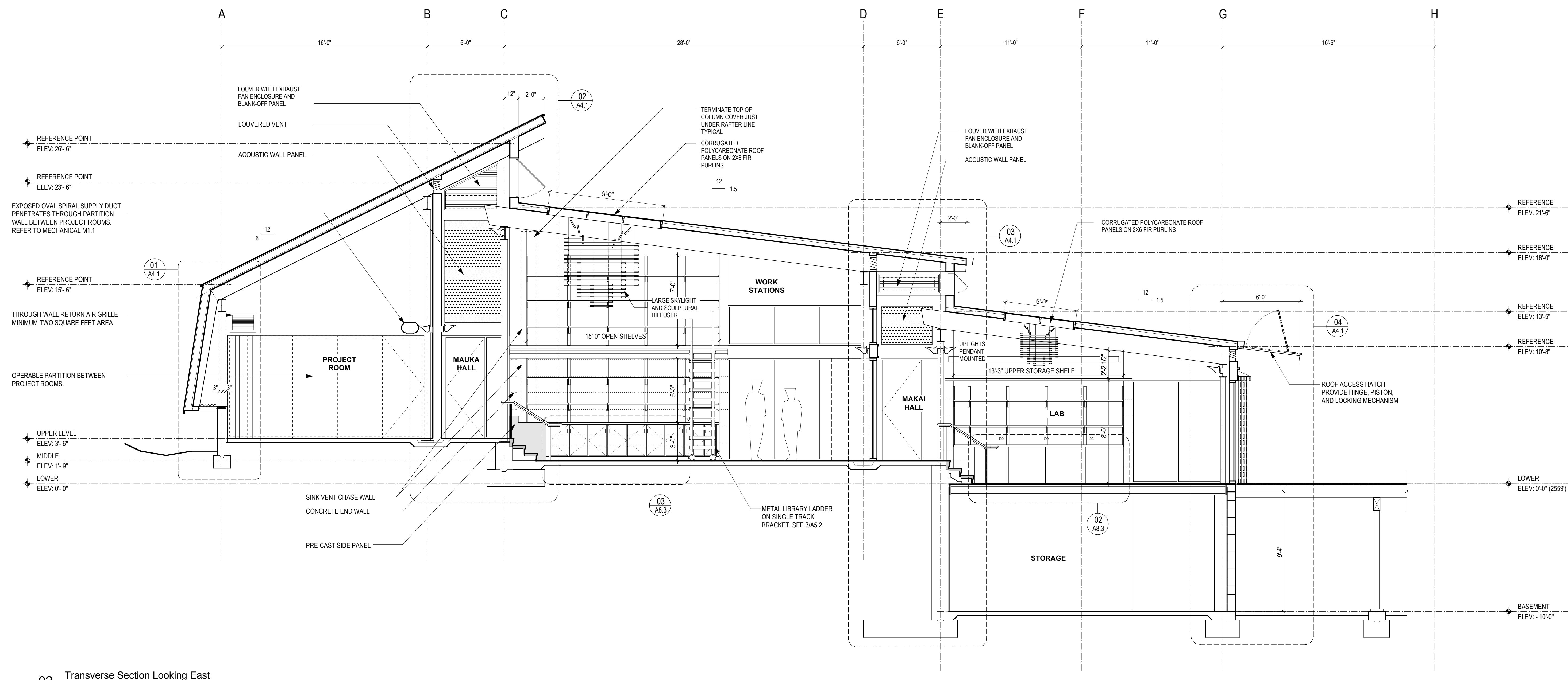
02 Transverse Section Looking East Scale: 1/4" = 1'-0"
