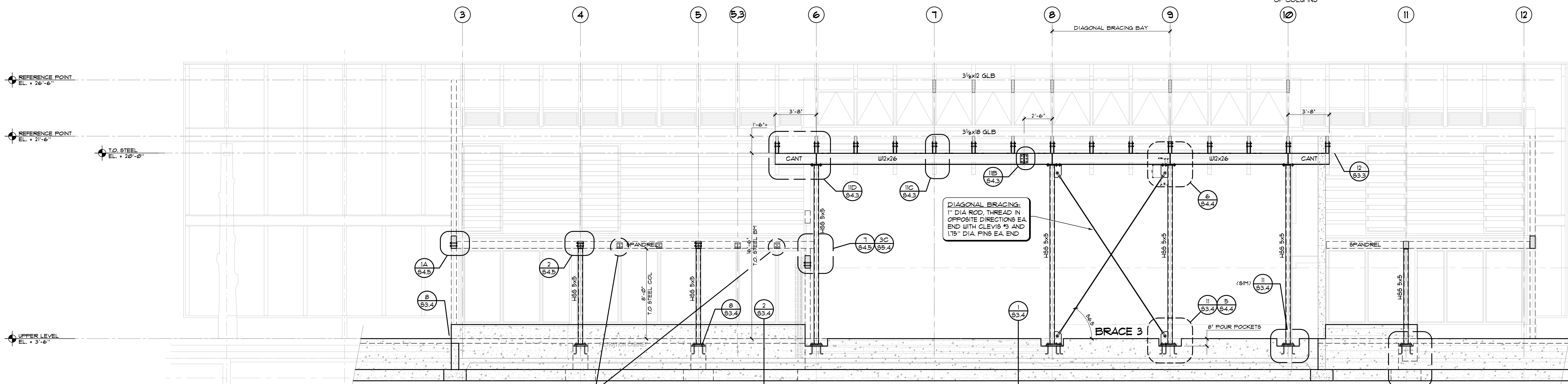
1 FRAMING ELEVATION: STRUCTURAL STEEL FRAMING ELEVATION ALONG GRID LINE (C) SCALE: 1/4" = 1'-0"
