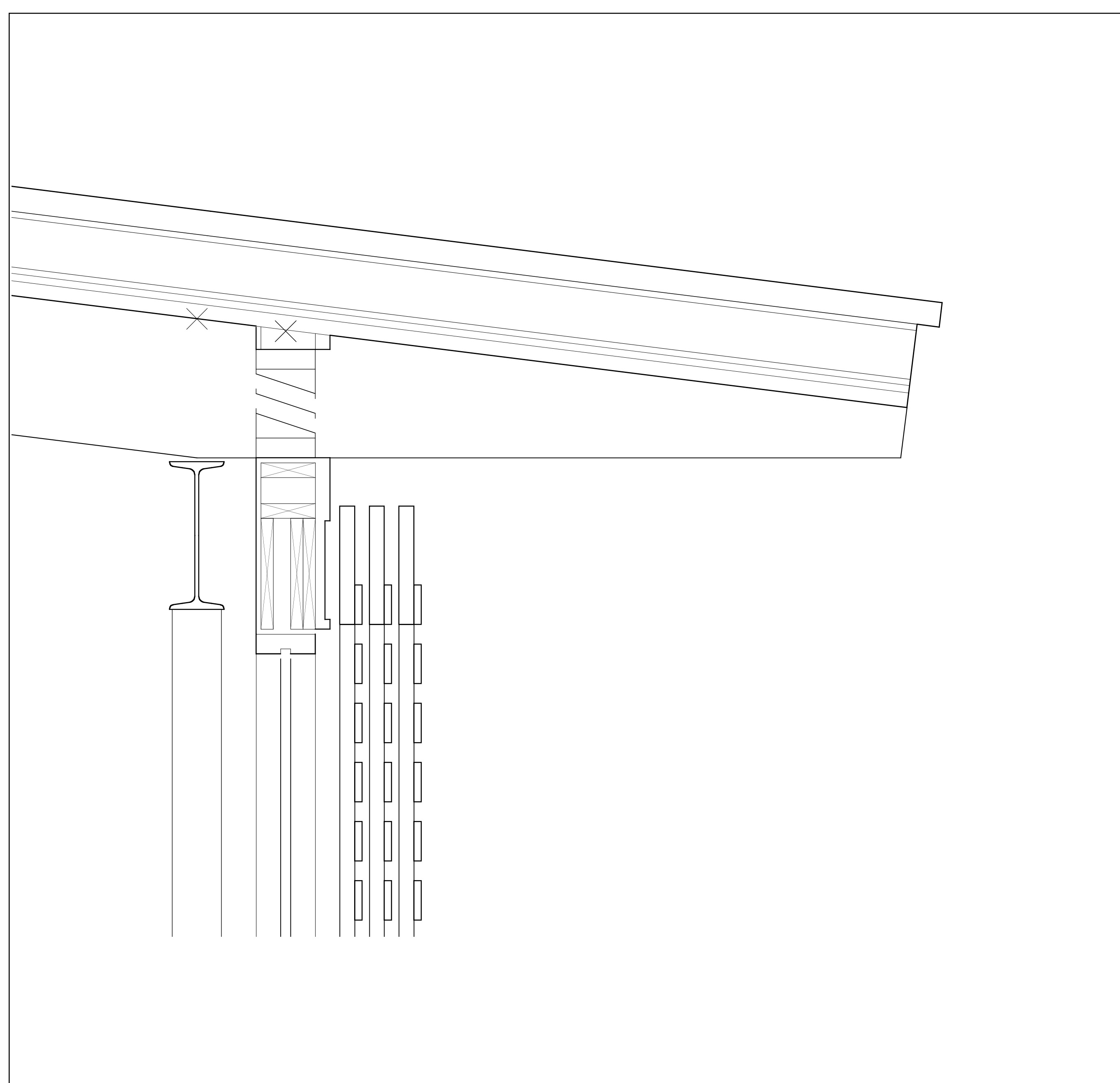
RAFTER TAIL DETAIL 7
