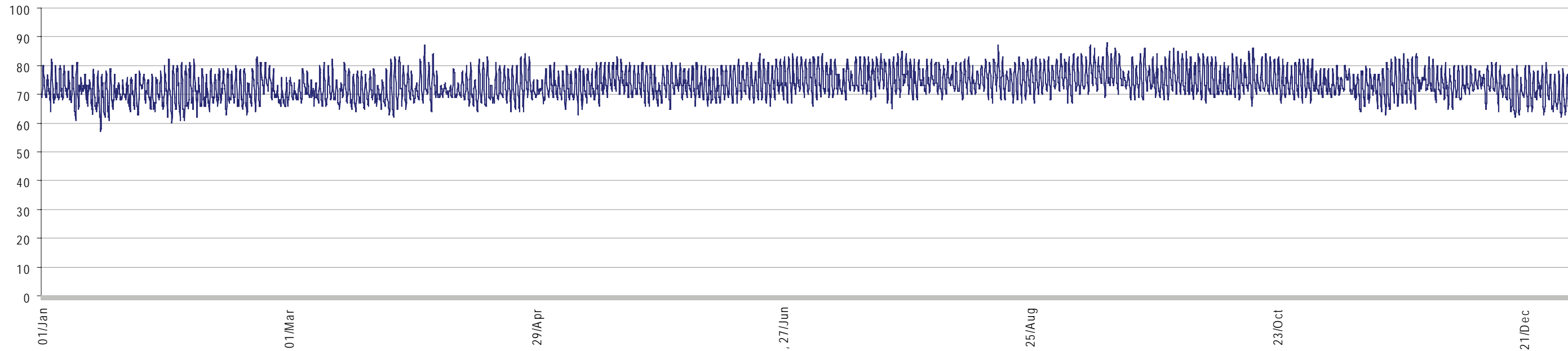
ANNUAL TEMPERATURE (Degree F)
