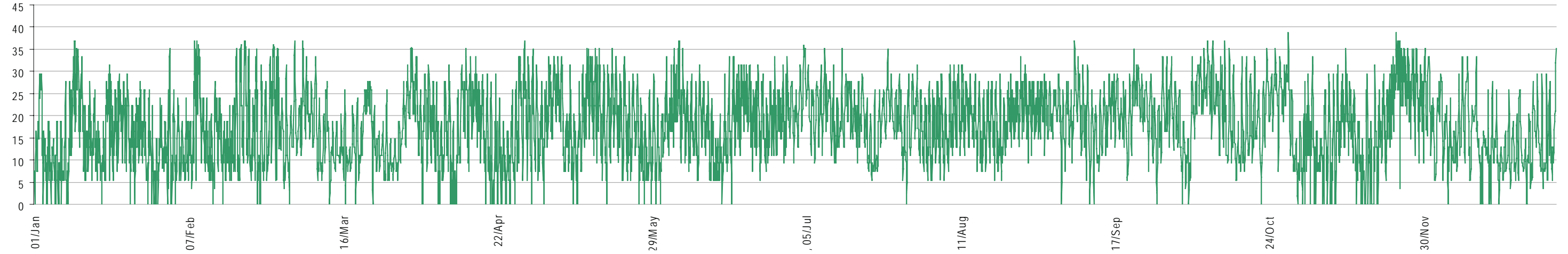
ANNUAL WIND SPEED (mph)
