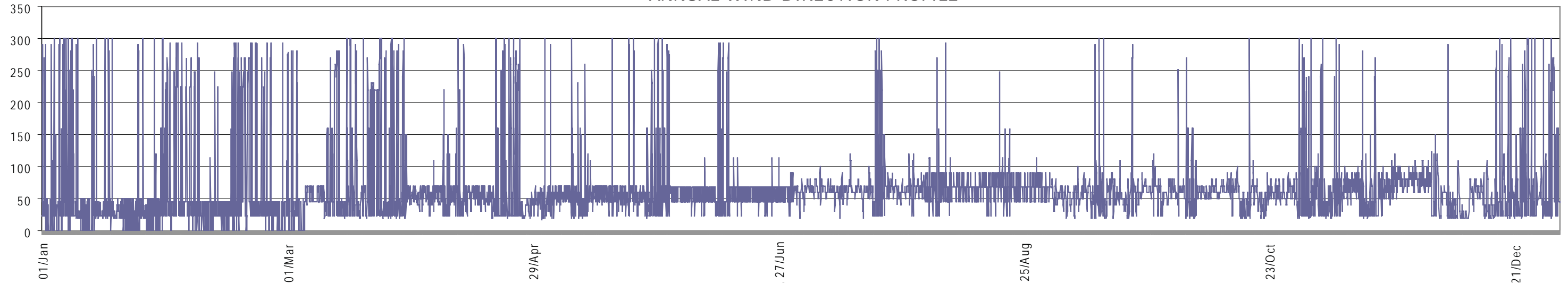
ANNUAL WIND DIRECTION PROFILE
