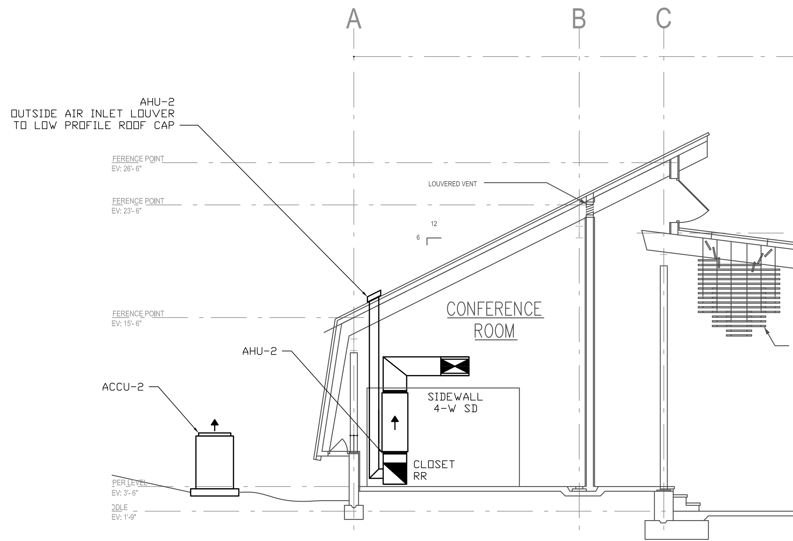
(A) SECTION B-B SCALE: 1/4" = 1 FT
