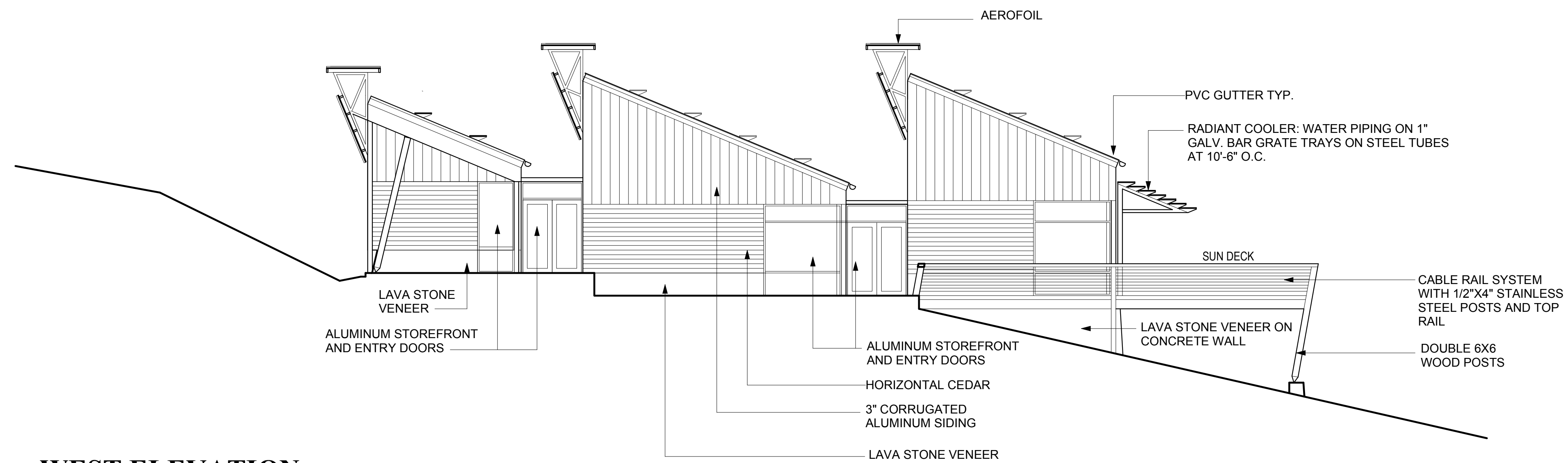
WEST ELEVATION
