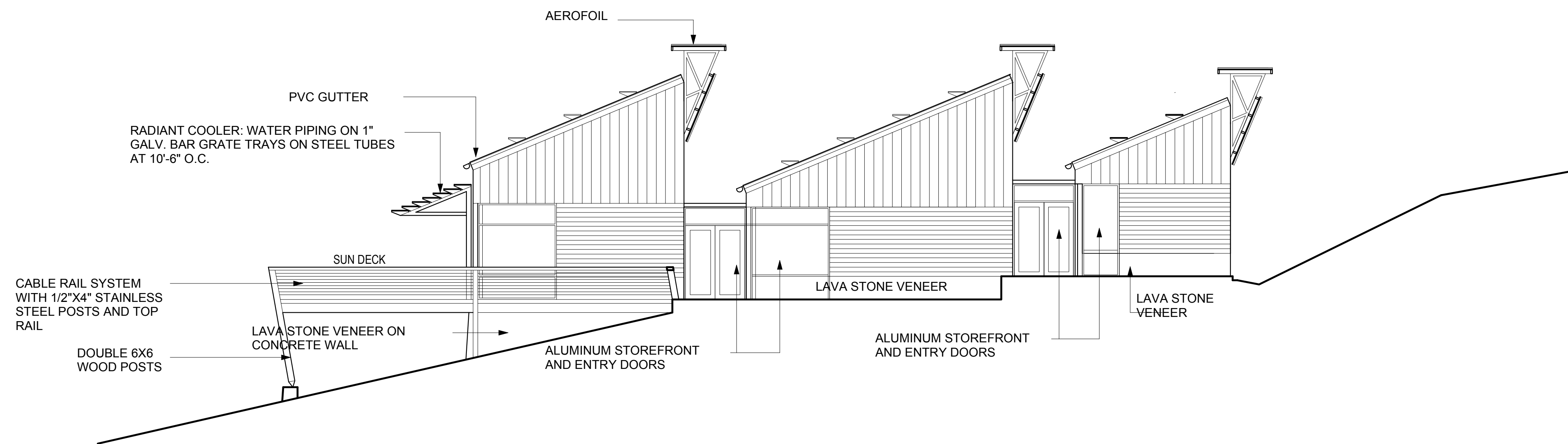
EAST ELEVATION
