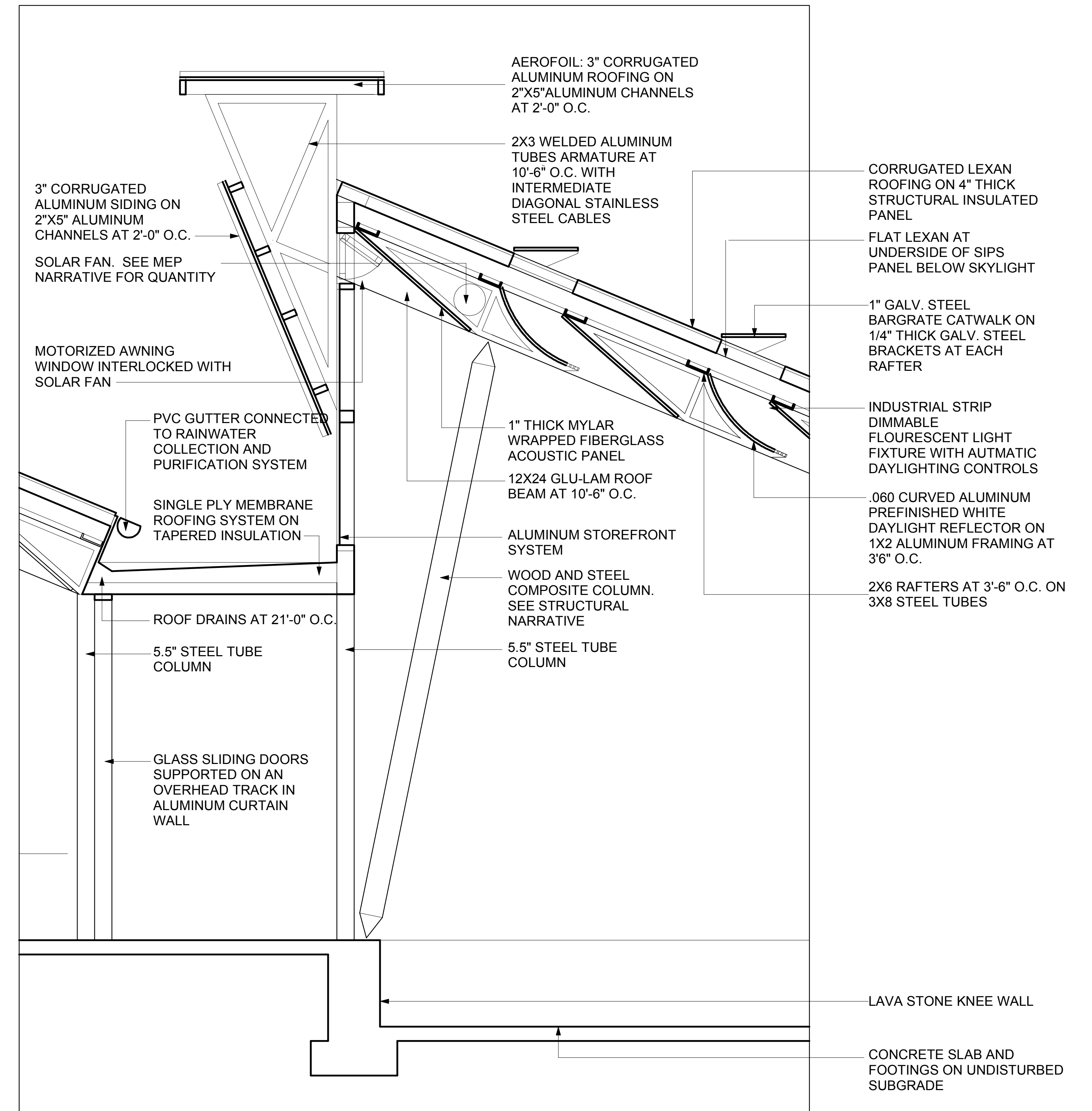
CROSS SECTION DETAIL
