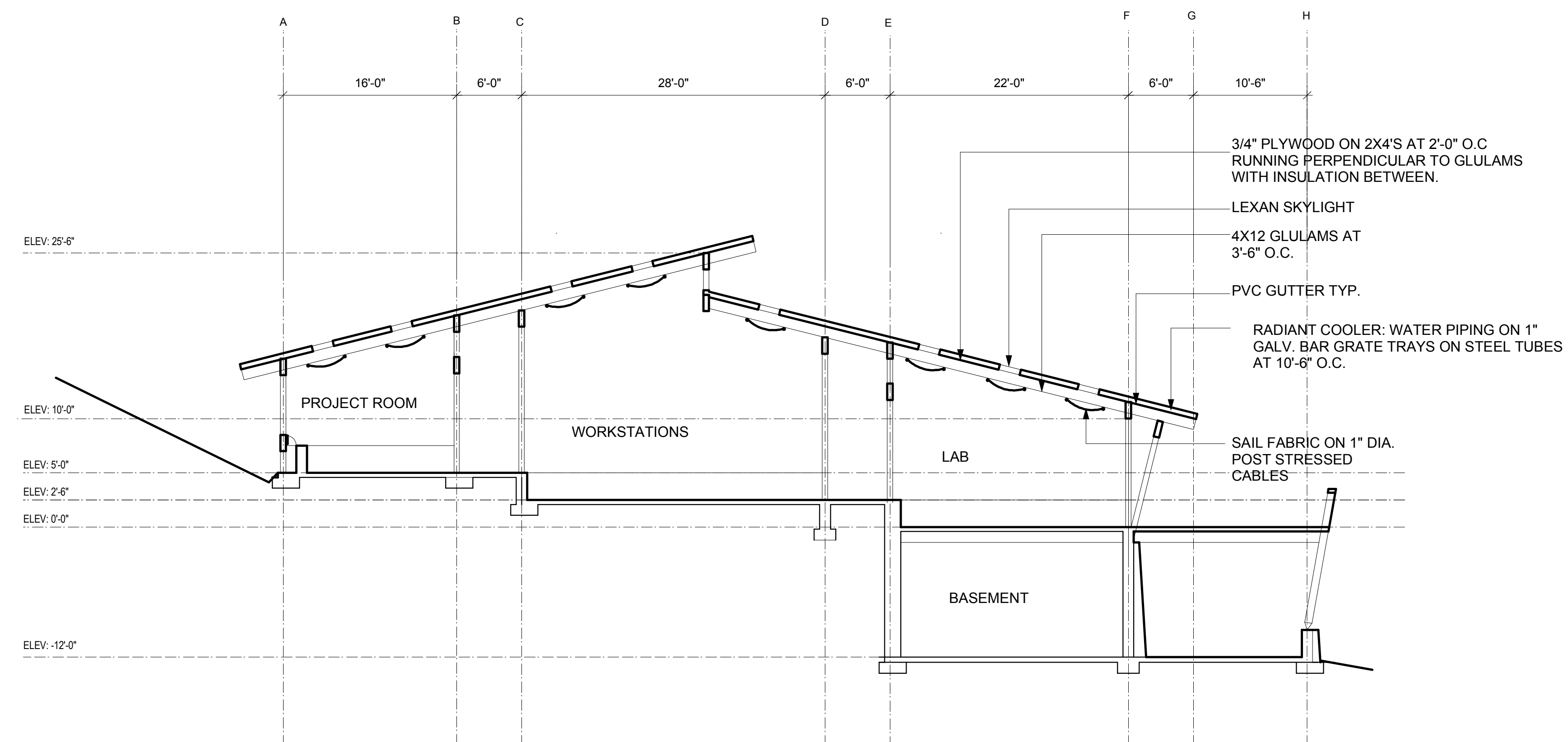
CROSS SECTION AT WORK STATIONS
