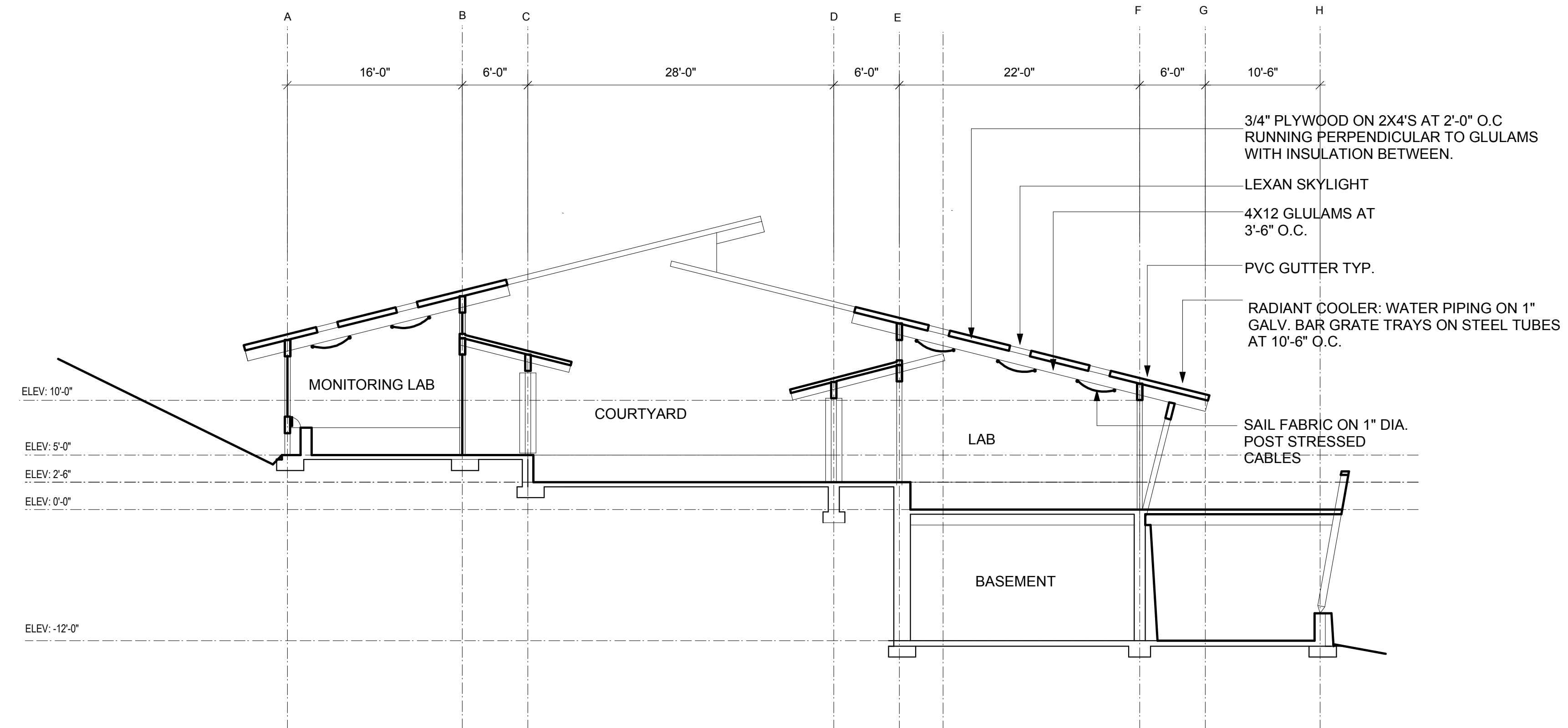
CROSS SECTION AT COURTYARD
